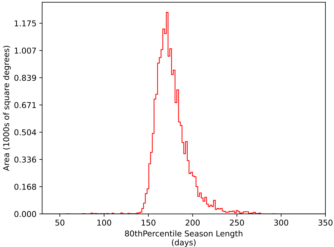
baseline_v3.5_10yrs WFD i band: 80thPercentile Season Length
