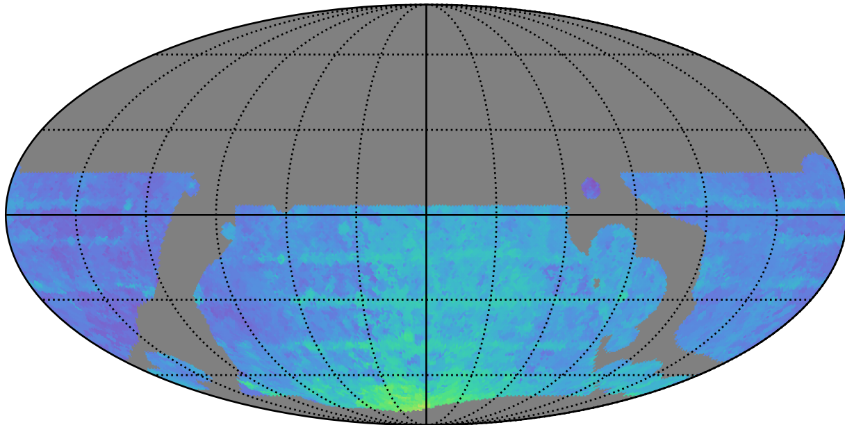
baseline_v3.5_10yrs WFD all bands: 80thPercentile Season Length
