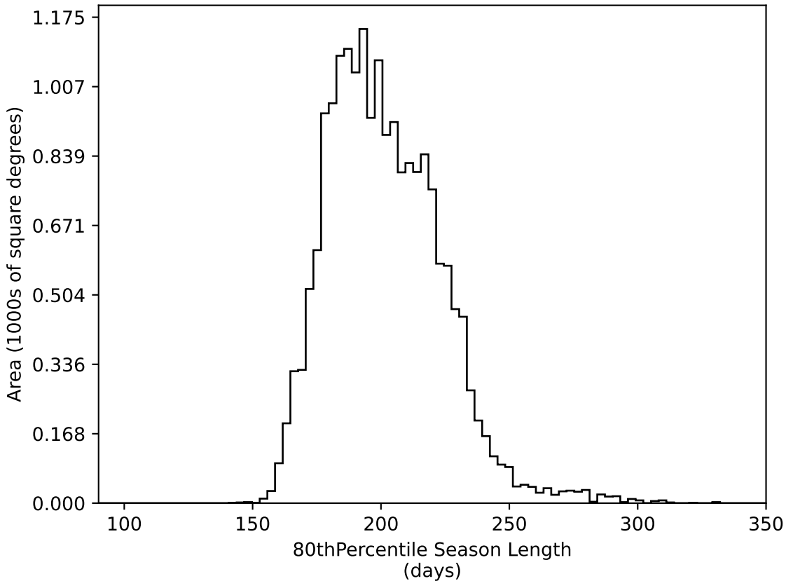
baseline_v3.5_10yrs WFD all bands: 80thPercentile Season Length
