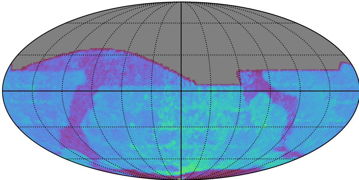
baseline_v3.5_10yrs All sky z band: 80thPercentile Season Length
