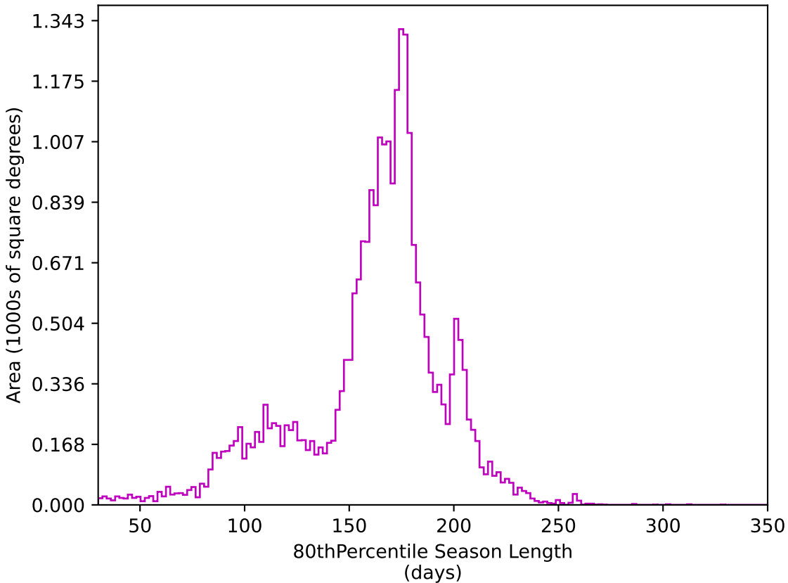
baseline_v3.5_10yrs All sky z band: 80thPercentile Season Length
