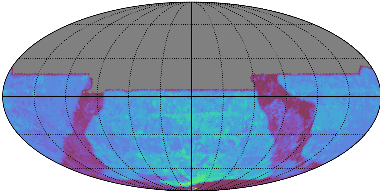
baseline_v3.5_10yrs All sky y band: 80thPercentile Season Length
