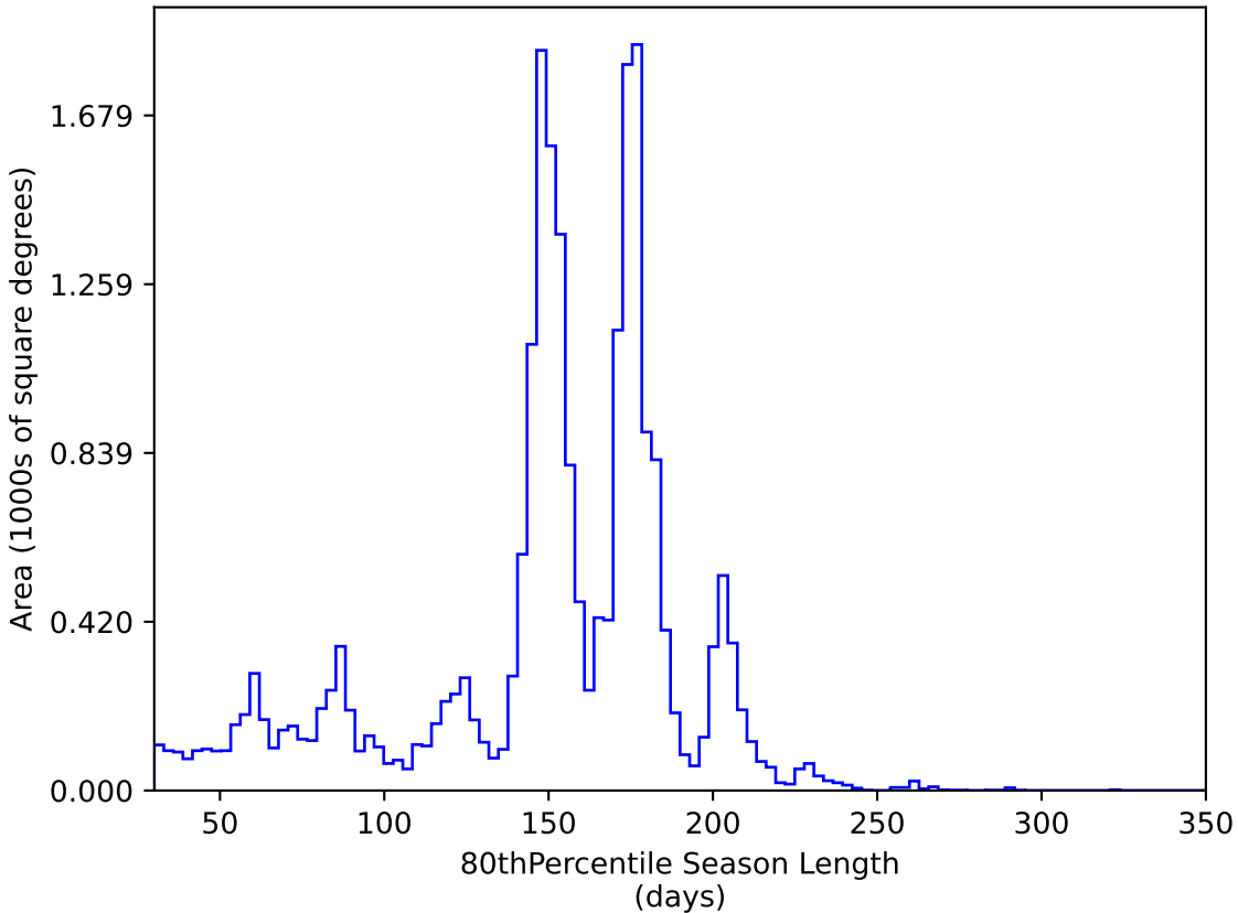
baseline_v3.5_10yrs All sky y band: 80thPercentile Season Length
