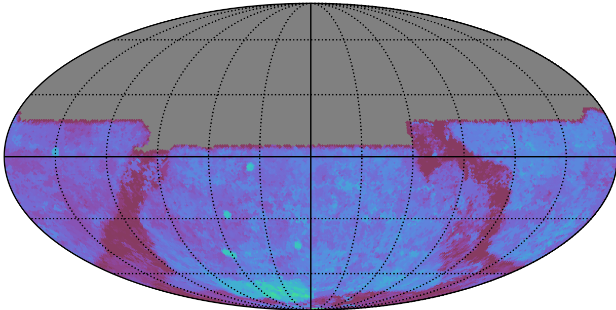
baseline_v3.5_10yrs All sky u band: 80thPercentile Season Length
