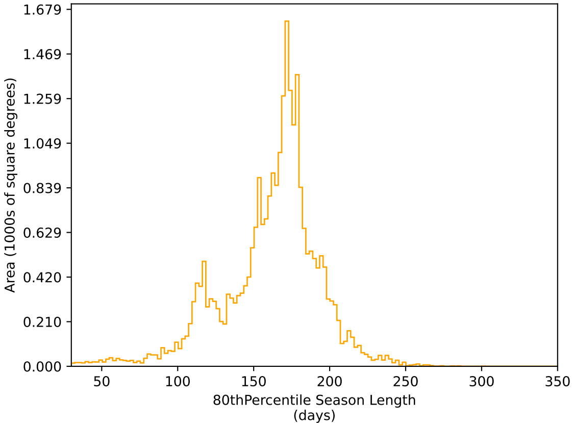
baseline_v3.5_10yrs All sky r band: 80thPercentile Season Length
