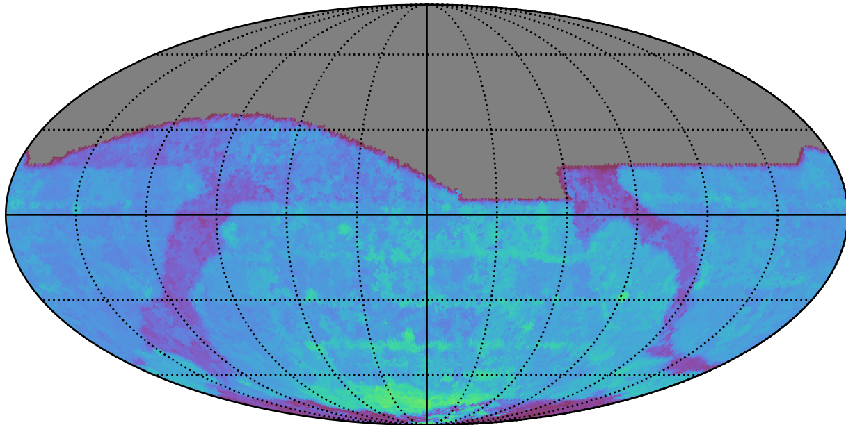
baseline_v3.5_10yrs All sky i band: 80thPercentile Season Length
