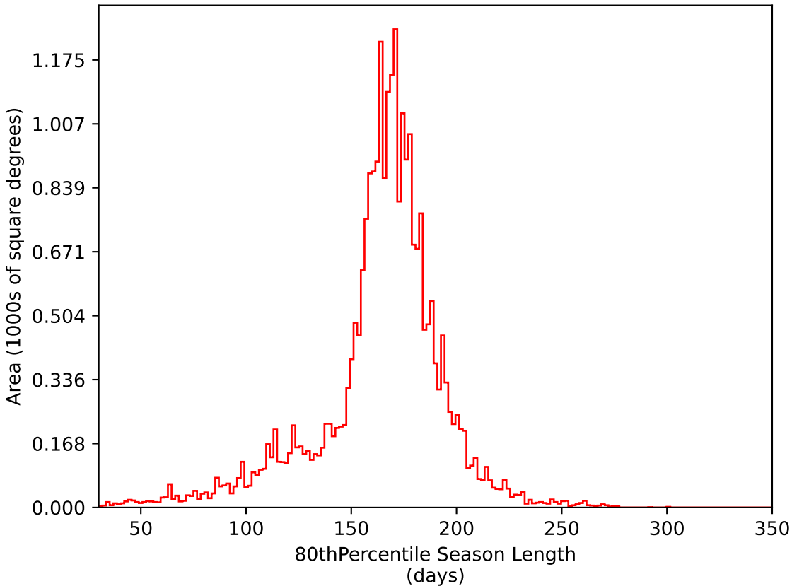
baseline_v3.5_10yrs All sky i band: 80thPercentile Season Length
