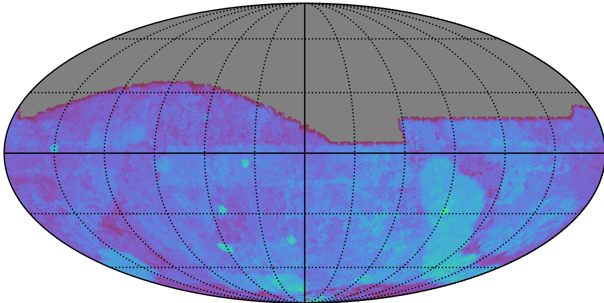
baseline_v3.5_10yrs All sky g band: 80thPercentile Season Length
