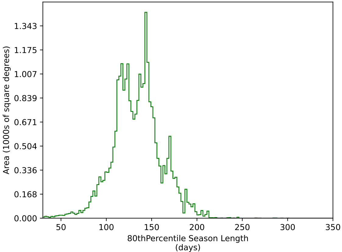
baseline_v3.5_10yrs All sky g band: 80thPercentile Season Length
