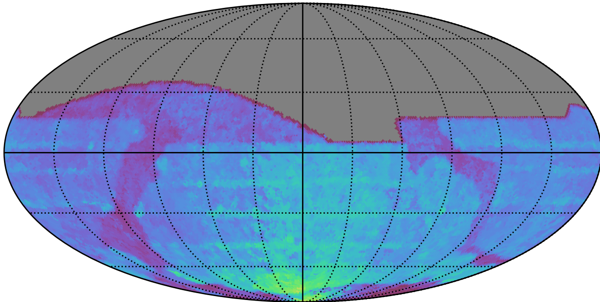
baseline_v3.5_10yrs All sky all bands: 80thPercentile Season Length
