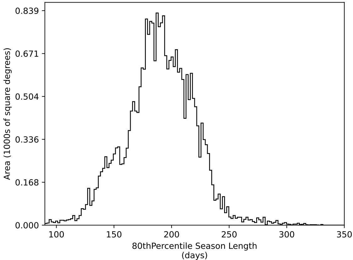
baseline_v3.5_10yrs All sky all bands: 80thPercentile Season Length
