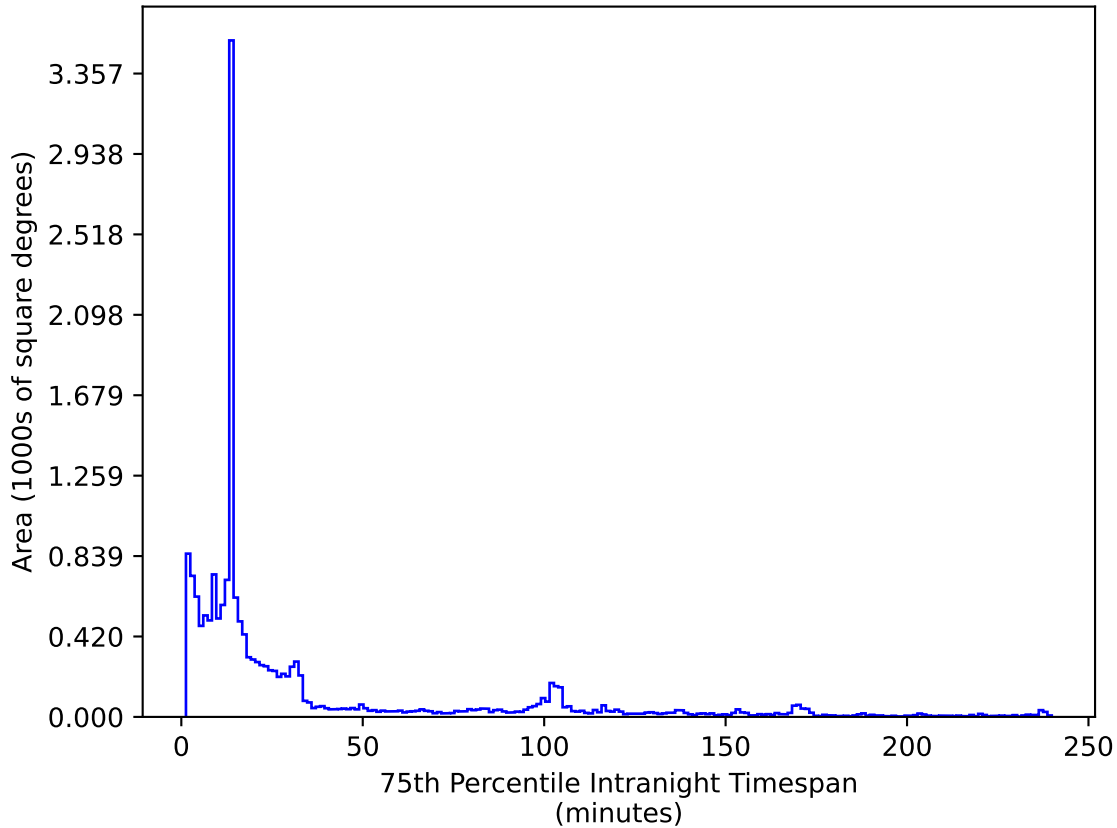
baseline_v3.5_10yrs WFD z band: 75th Percentile Intranight Timespan
