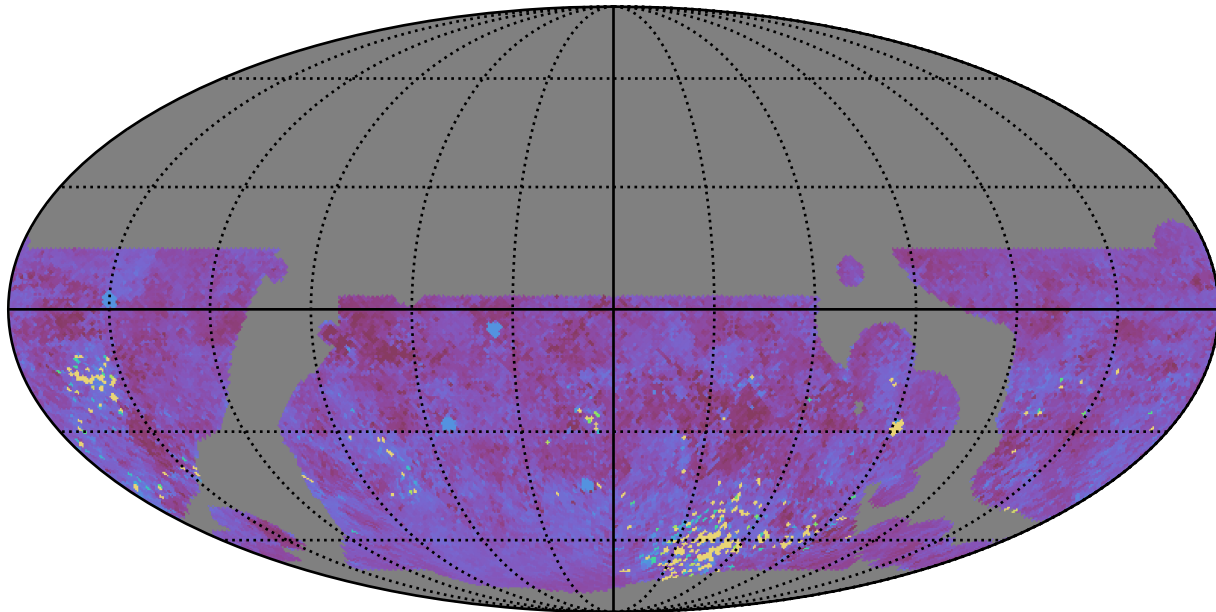
baseline_v3.5_10yrs WFD ug bands: 75th Percentile Intranight Timespan
