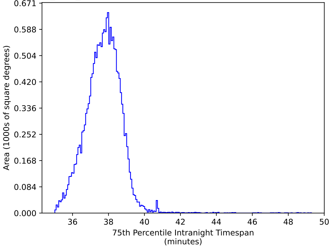
baseline_v3.5_10yrs WFD ug bands: 75th Percentile Intranight Timespan
