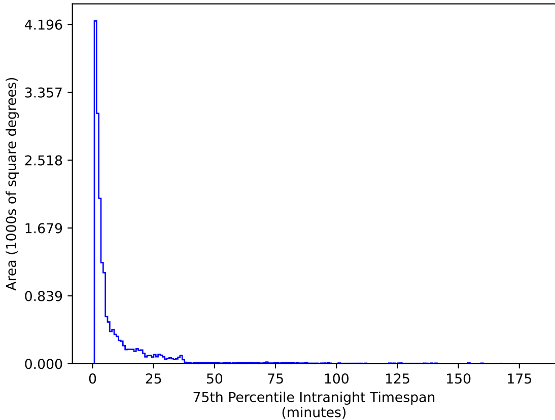
baseline_v3.5_10yrs WFD u band: 75th Percentile Intranight Timespan
