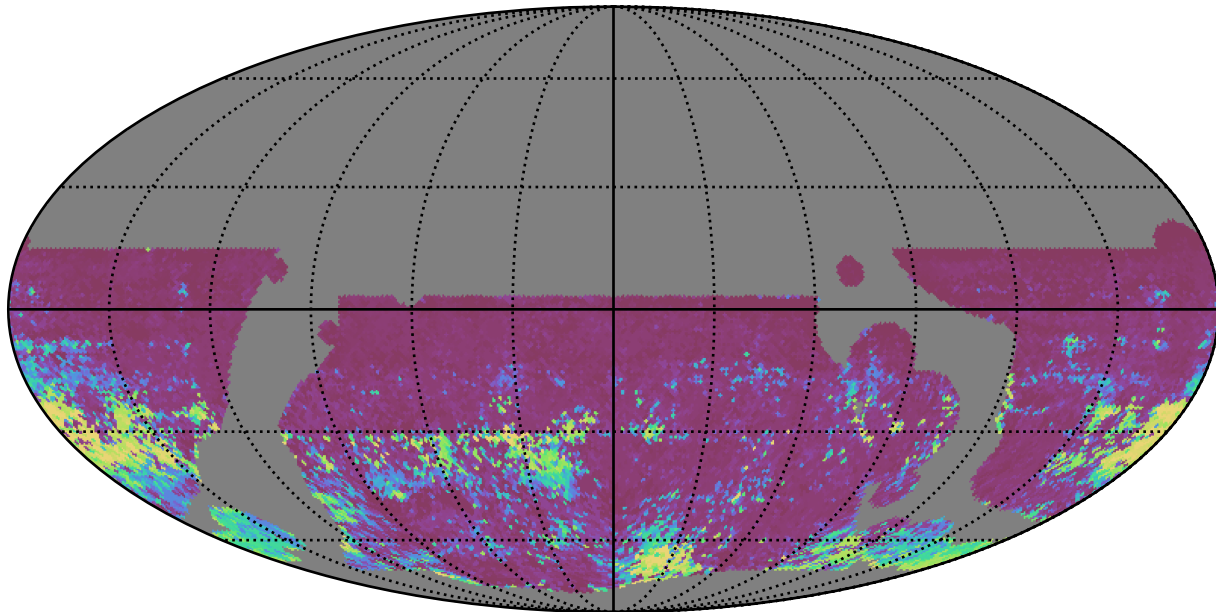
baseline_v3.5_10yrs WFD r band: 75th Percentile Intranight Timespan
