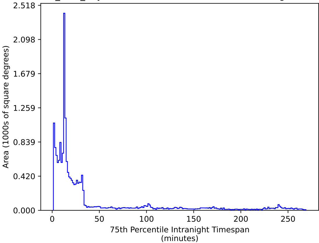
baseline_v3.5_10yrs WFD r band: 75th Percentile Intranight Timespan
