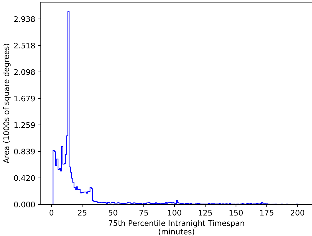
baseline_v3.5_10yrs WFD i band: 75th Percentile Intranight Timespan
