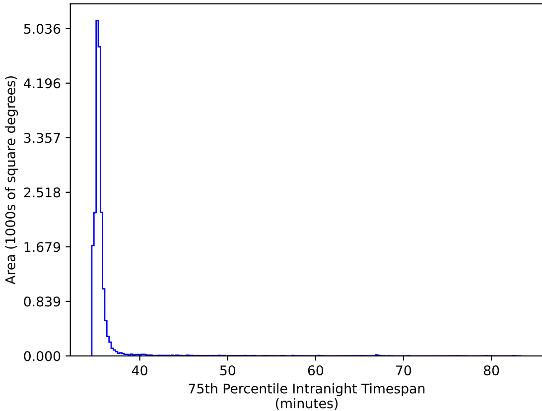
baseline_v3.5_10yrs WFD gr bands: 75th Percentile Intranight Timespan
