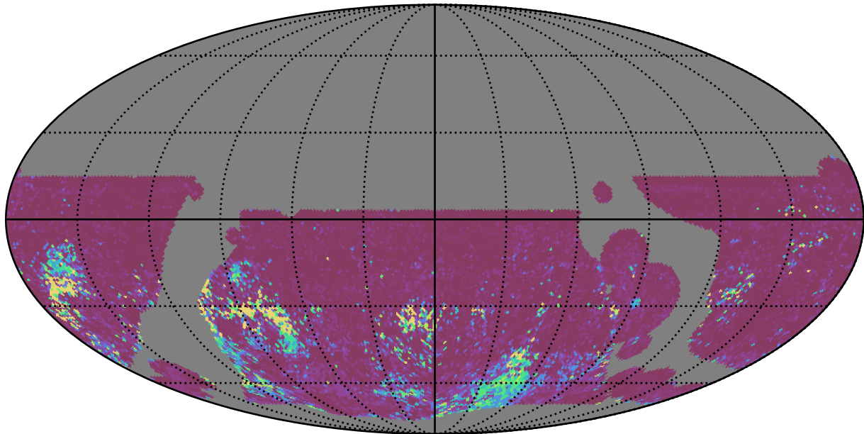
baseline_v3.5_10yrs WFD g band: 75th Percentile Intranight Timespan
