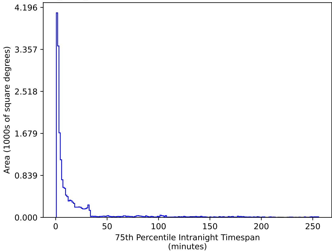
baseline_v3.5_10yrs WFD g band: 75th Percentile Intranight Timespan
