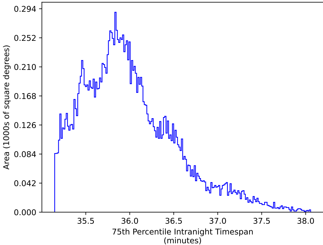
baseline_v3.5_10yrs WFD all bands: 75th Percentile Intranight Timespan
