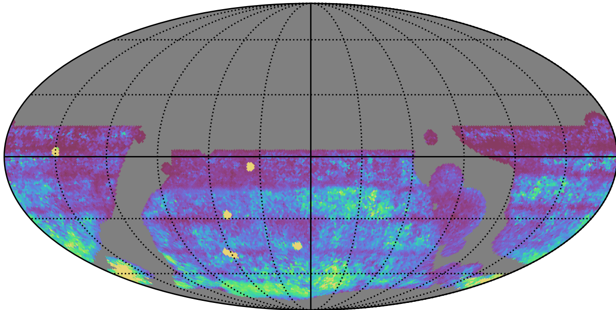
baseline_v3.5_10yrs WFD: 75th Percentile Intranight Timespan
