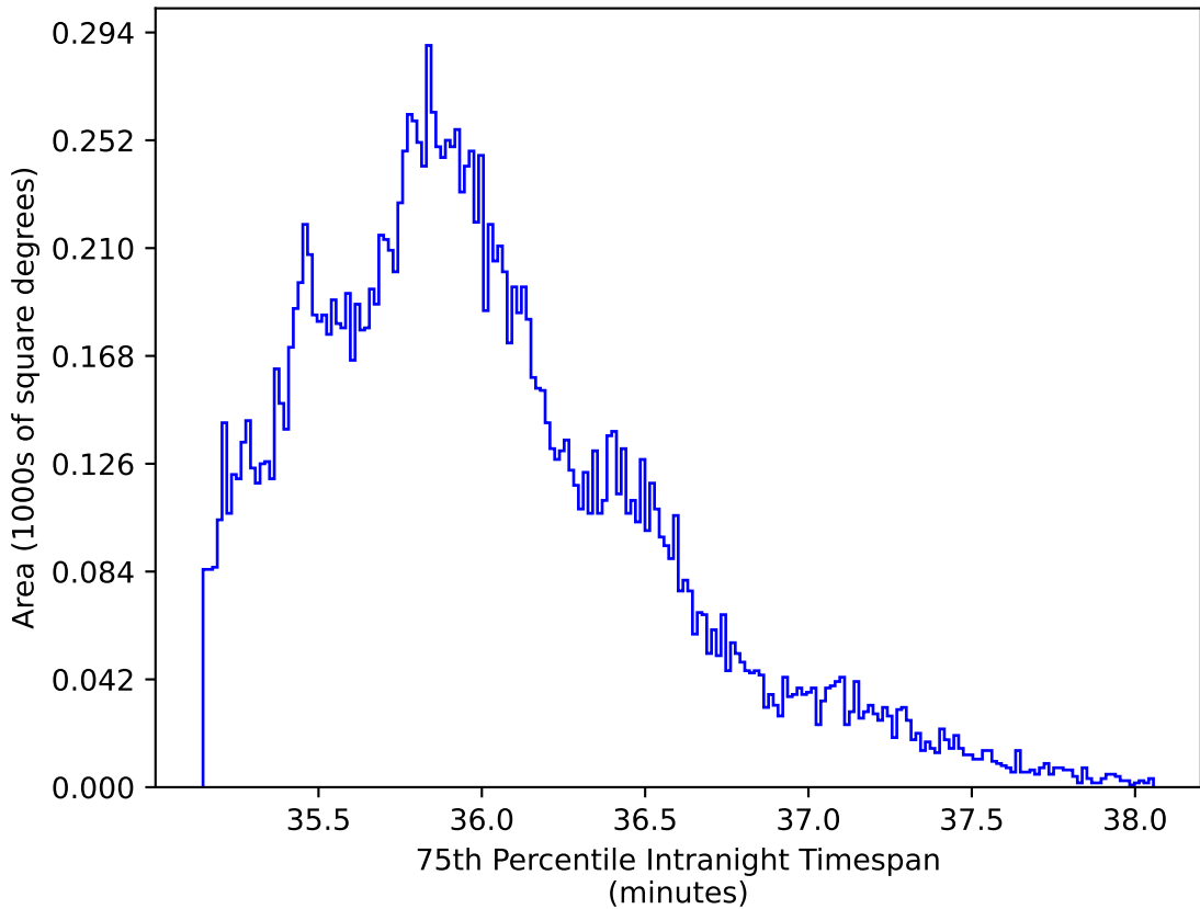
baseline_v3.5_10yrs WFD: 75th Percentile Intranight Timespan
