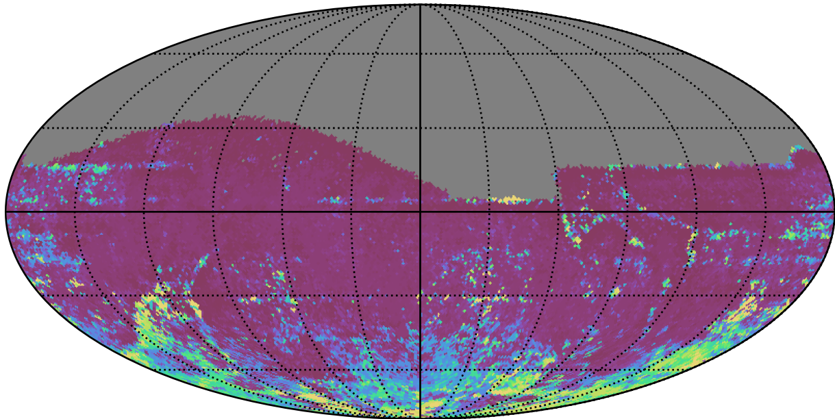
baseline_v3.5_10yrs All sky z band: 75th Percentile Intranight Timespan
