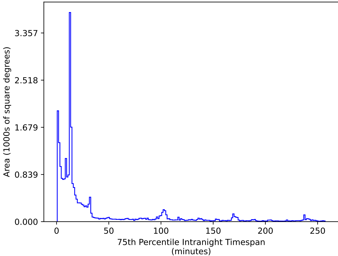
baseline_v3.5_10yrs All sky z band: 75th Percentile Intranight Timespan
