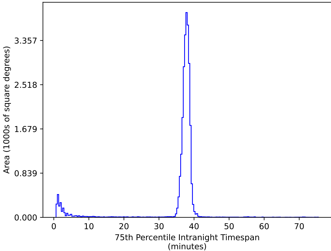
baseline_v3.5_10yrs All sky ug bands: 75th Percentile Intranight Timespan
