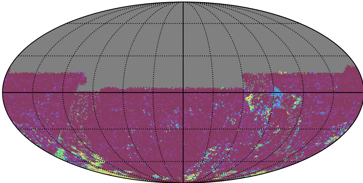
baseline_v3.5_10yrs All sky u band: 75th Percentile Intranight Timespan
