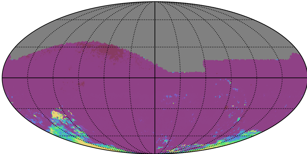
baseline_v3.5_10yrs All sky ri bands: 75th Percentile Intranight Timespan
