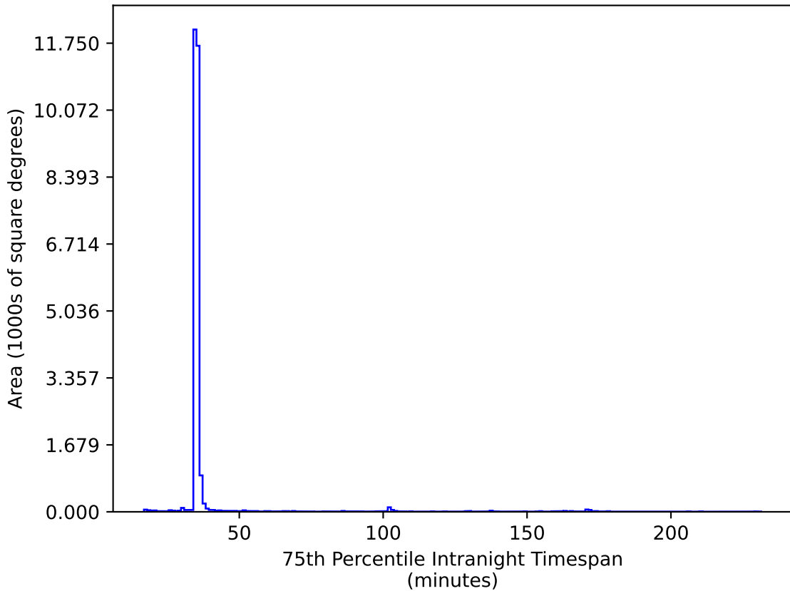
baseline_v3.5_10yrs All sky ri bands: 75th Percentile Intranight Timespan
