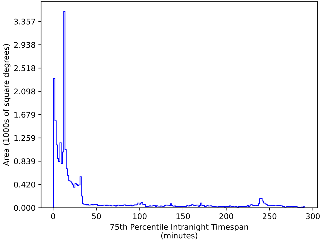
baseline_v3.5_10yrs All sky r band: 75th Percentile Intranight Timespan
