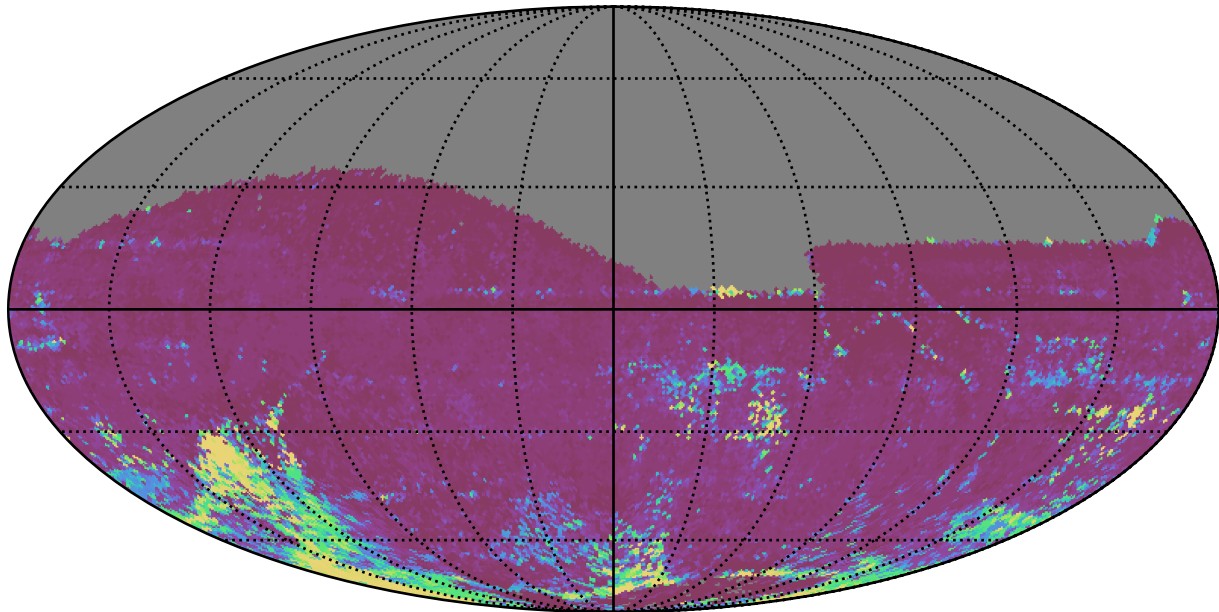
baseline_v3.5_10yrs All sky i band: 75th Percentile Intranight Timespan
