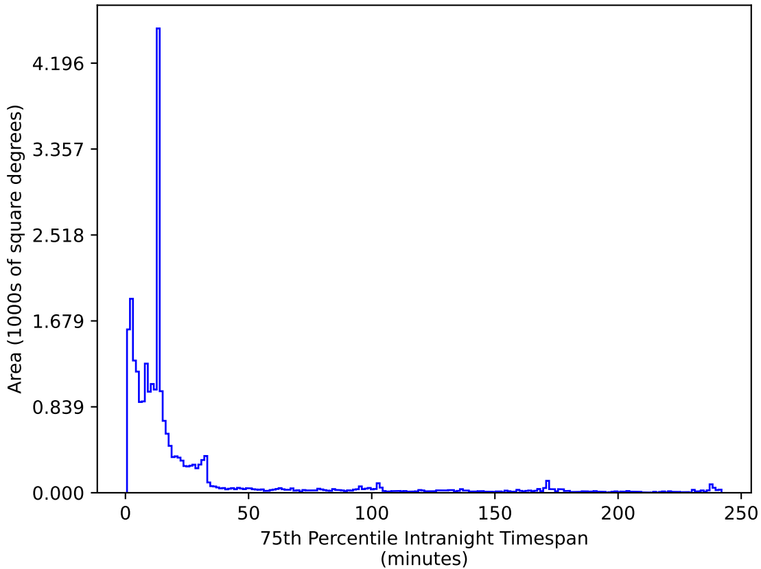
baseline_v3.5_10yrs All sky i band: 75th Percentile Intranight Timespan
