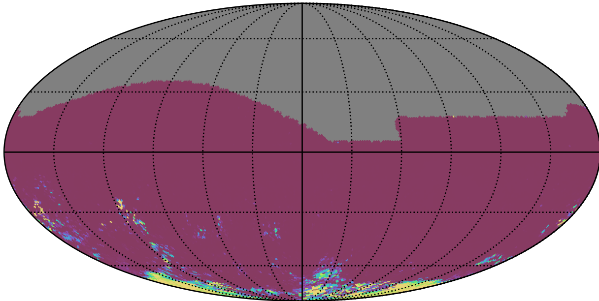
baseline_v3.5_10yrs All sky gr bands: 75th Percentile Intranight Timespan
