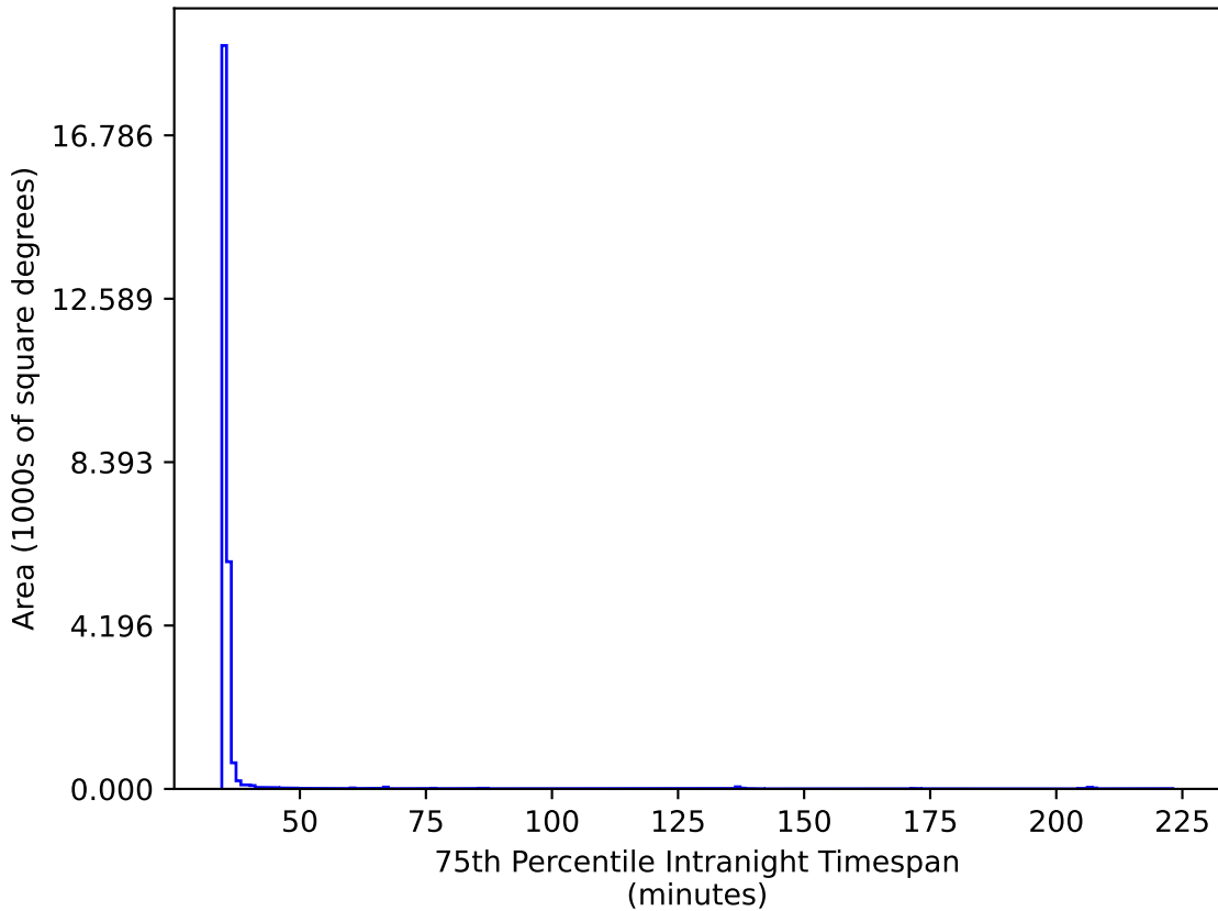
baseline_v3.5_10yrs All sky gr bands: 75th Percentile Intranight Timespan
