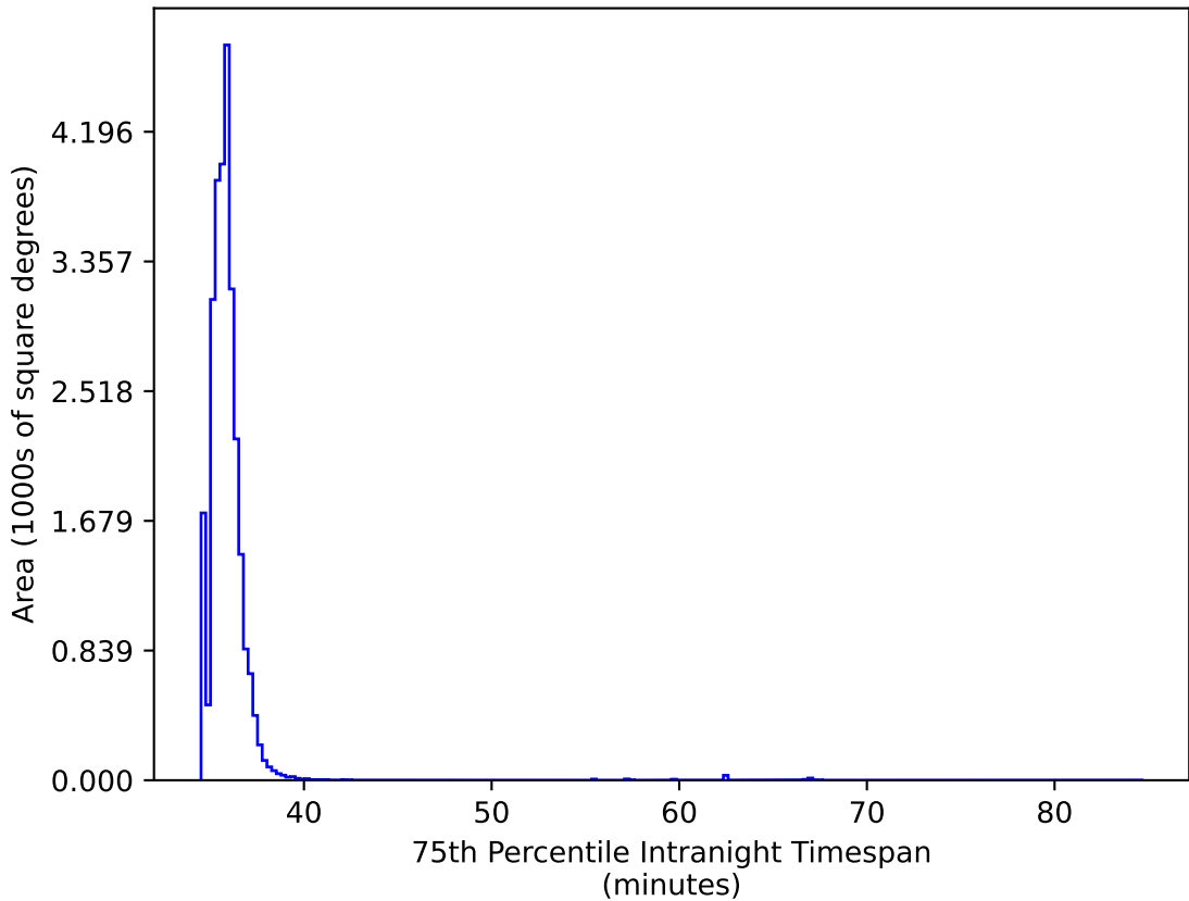
baseline_v3.5_10yrs All sky all bands: 75th Percentile Intranight Timespan
