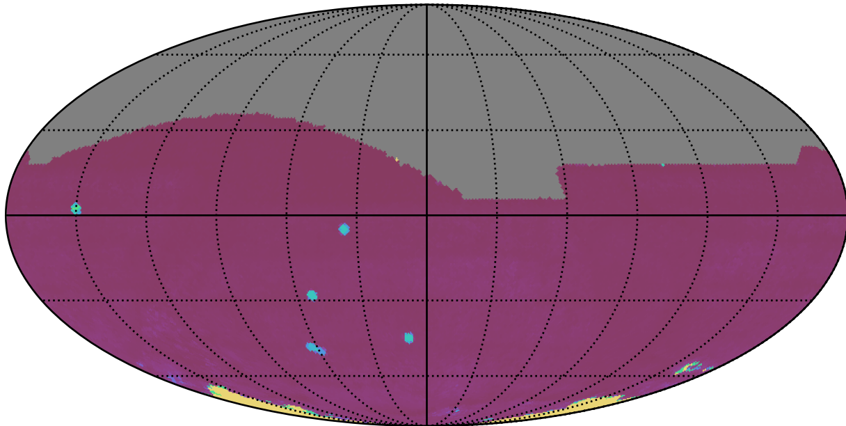
baseline_v3.5_10yrs All sky: 75th Percentile Intranight Timespan
