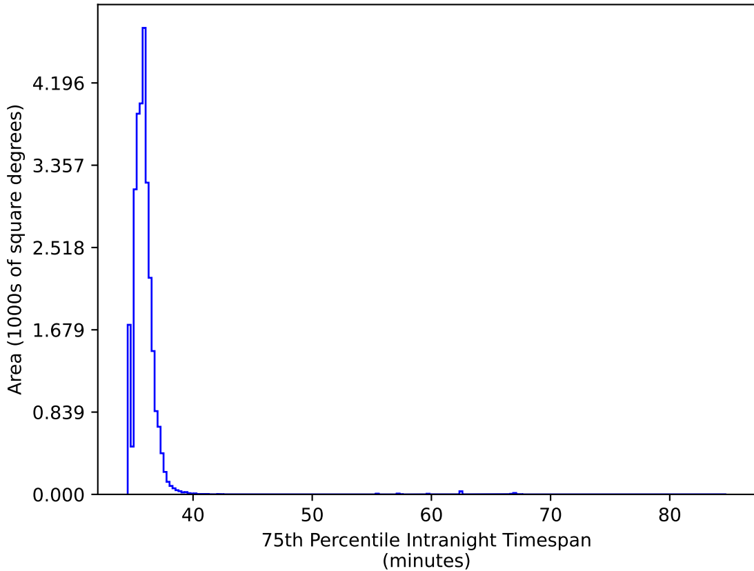
baseline_v3.5_10yrs All sky: 75th Percentile Intranight Timespan
