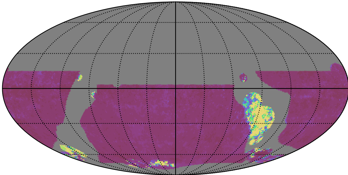
baseline_v3.5_10yrs WFD y band: 20thPercentile Inter-Night Gap
