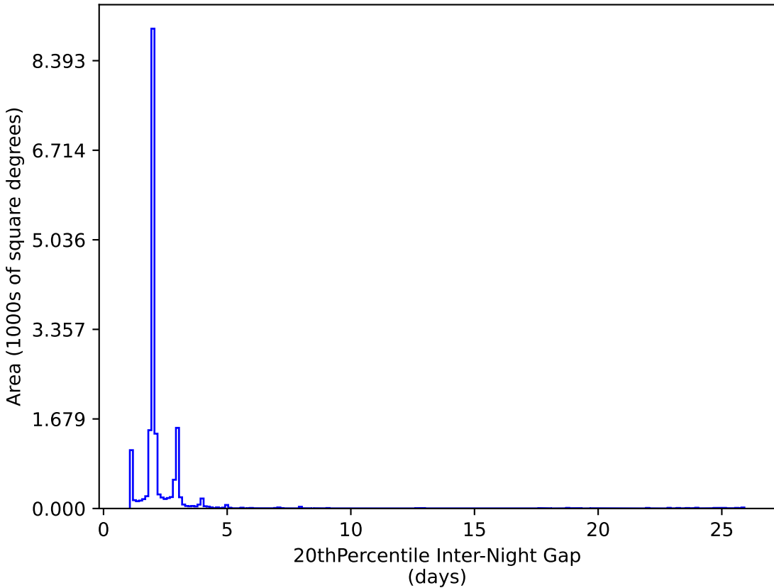
baseline_v3.5_10yrs WFD y band: 20thPercentile Inter-Night Gap
