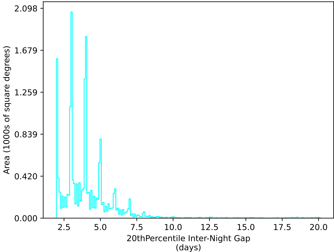
baseline_v3.5_10yrs WFD u band: 20thPercentile Inter-Night Gap
