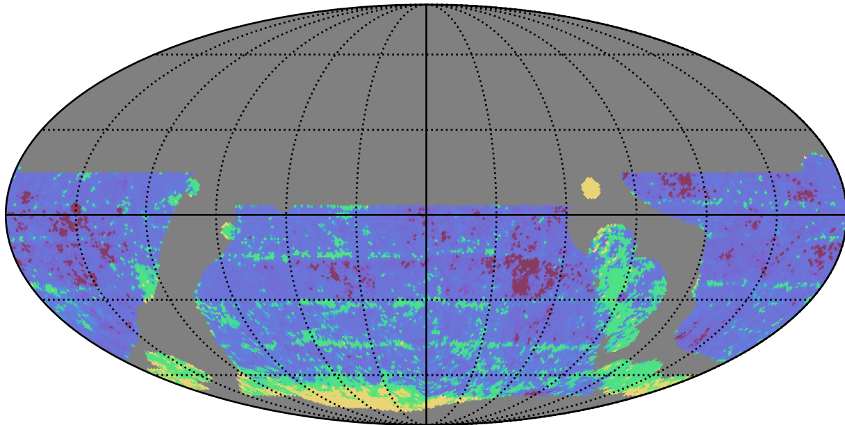
baseline_v3.5_10yrs WFD r band: 20thPercentile Inter-Night Gap
