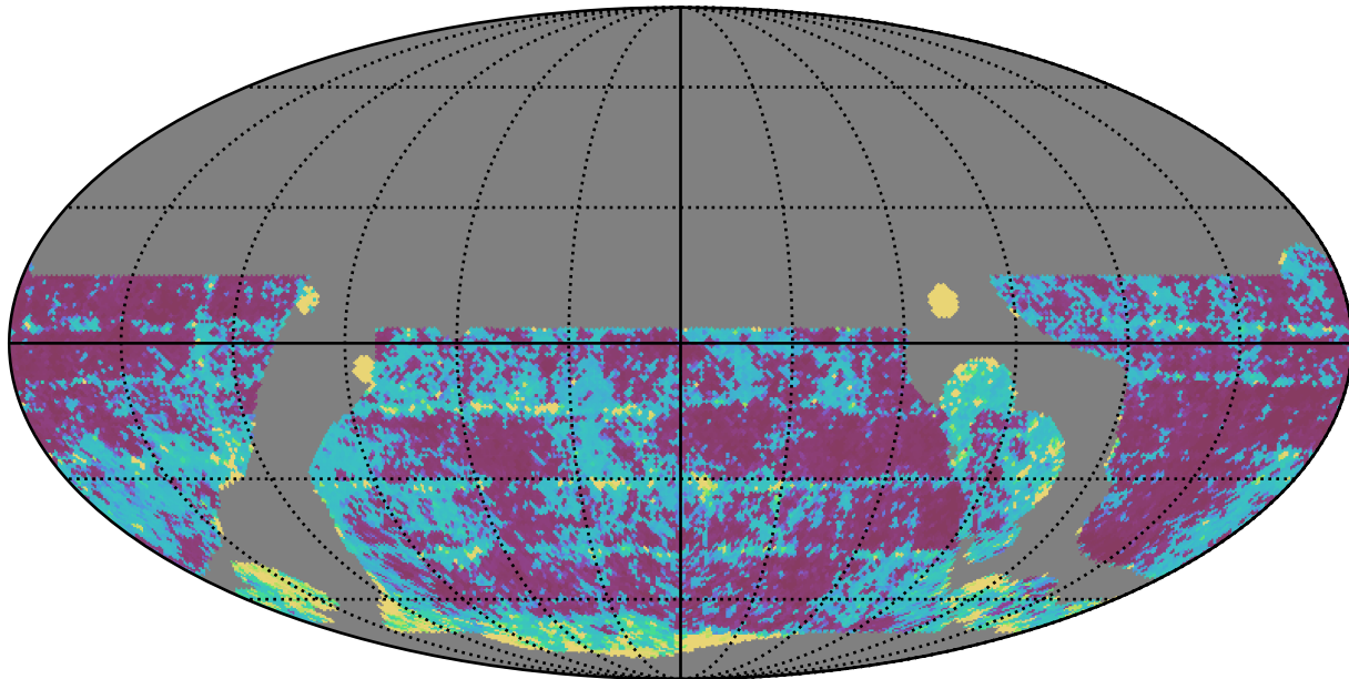
baseline_v3.5_10yrs WFD i band: 20thPercentile Inter-Night Gap
