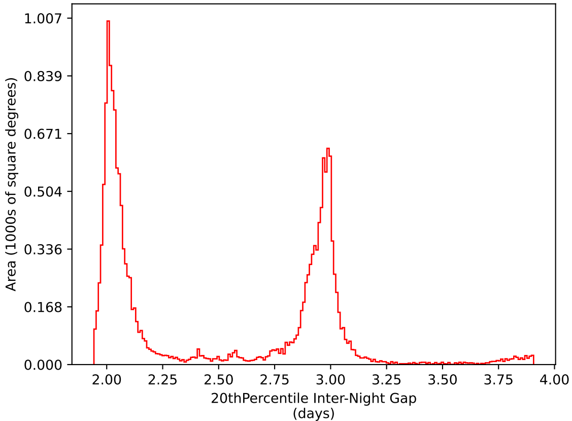
baseline_v3.5_10yrs WFD i band: 20thPercentile Inter-Night Gap
