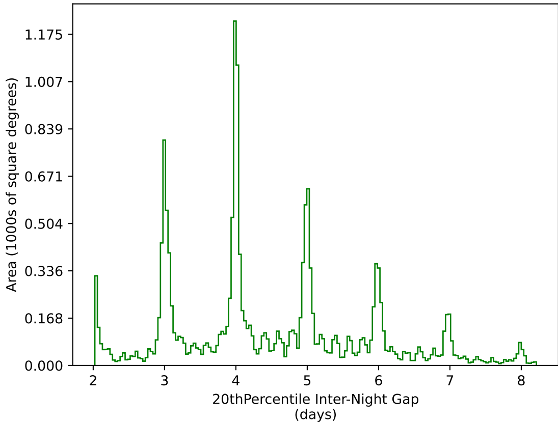
baseline_v3.5_10yrs WFD g band: 20thPercentile Inter-Night Gap
