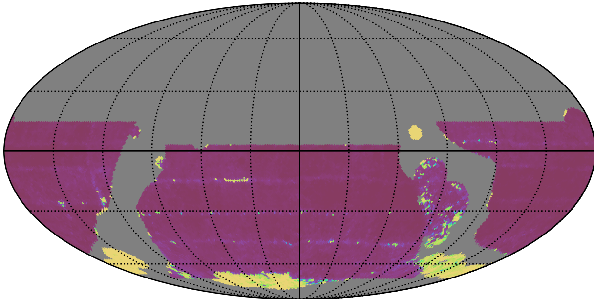
baseline_v3.5_10yrs WFD all bands: 20thPercentile Inter-Night Gap
